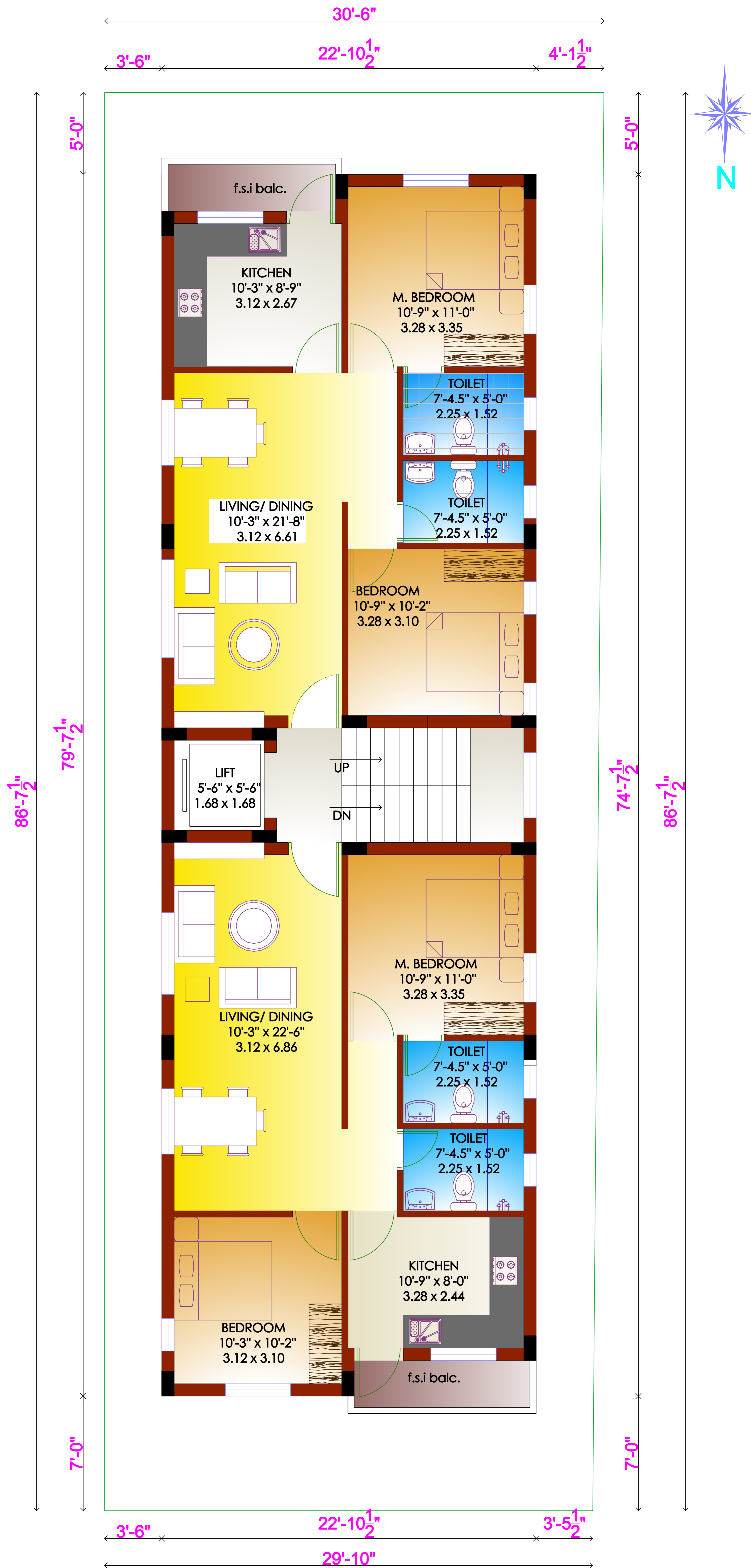
TYPICAL FLOOR PLAN (FIRST AND SECOND FLOOR PLAN)
